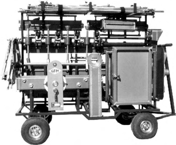
GF-6 crane transporter
